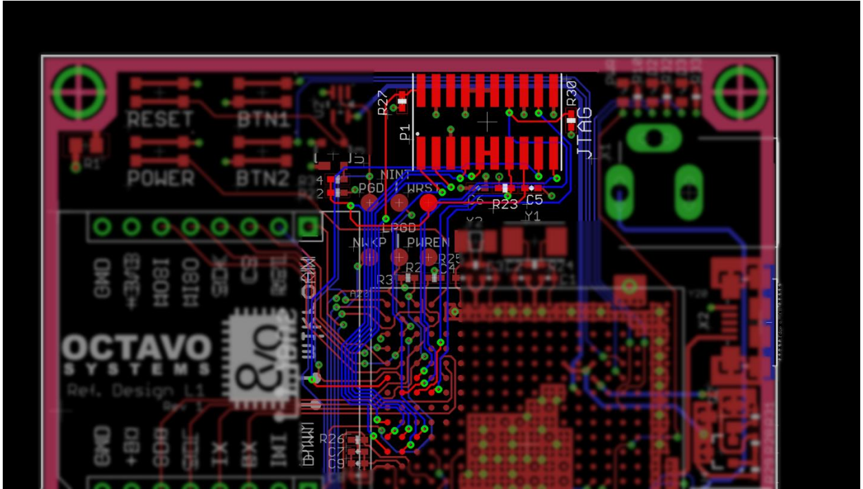
Figure 53 JTAG layout
