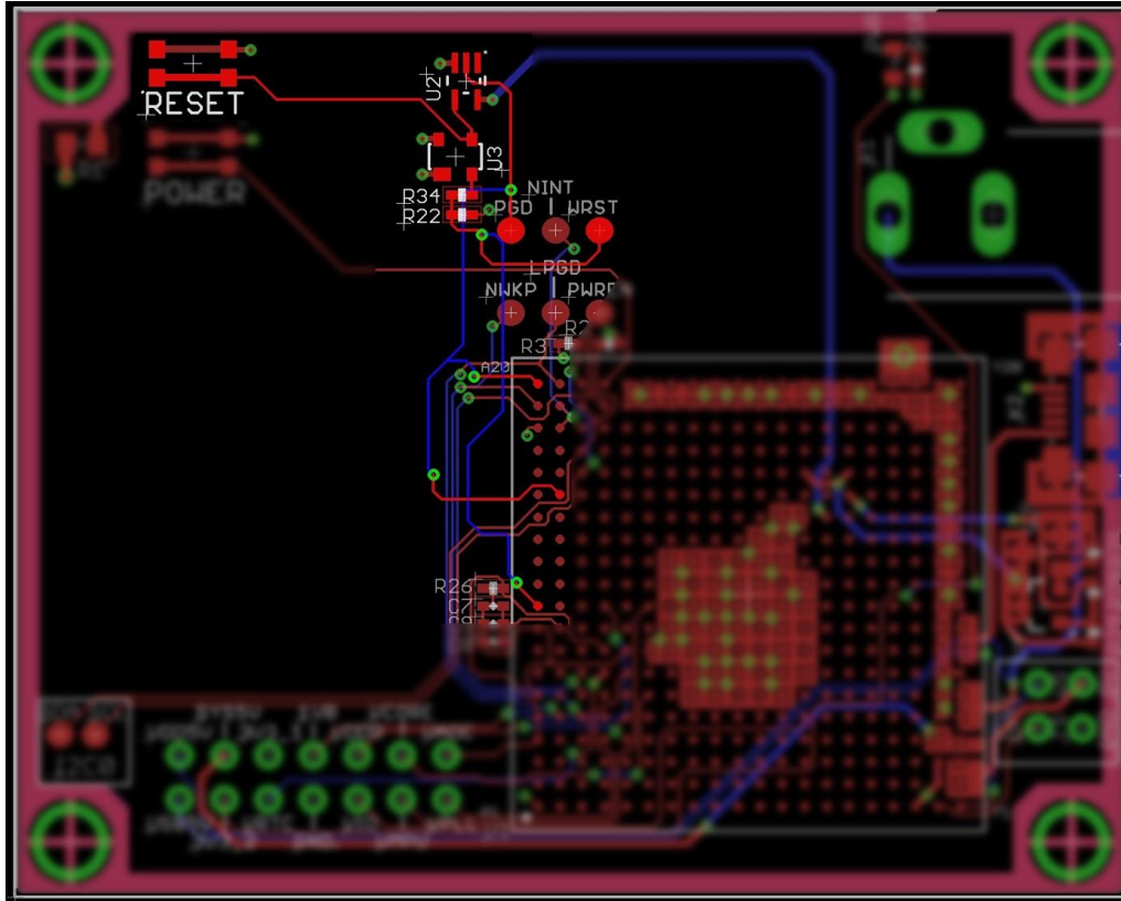
Figure 45 Reset circuitry layout
