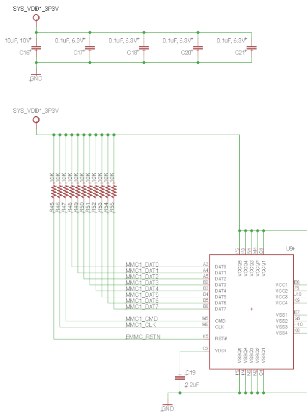
Figure 98 eMMC Circuitry
