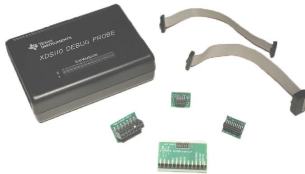
Figure 69 XDS110 Debugger
