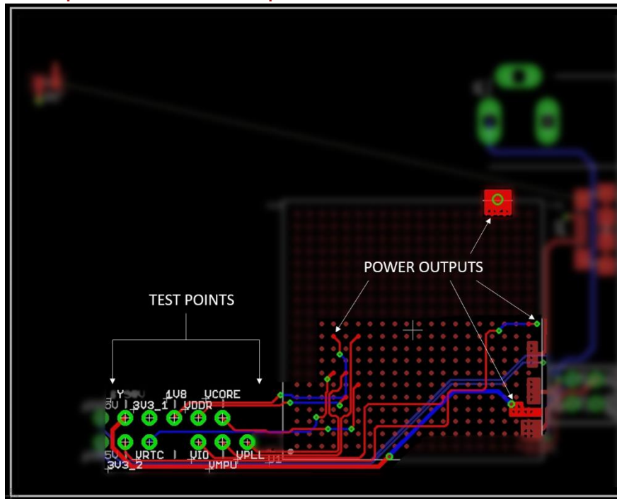
Figure 12 OSD335x layout for power output pins and test points on internal power rails
