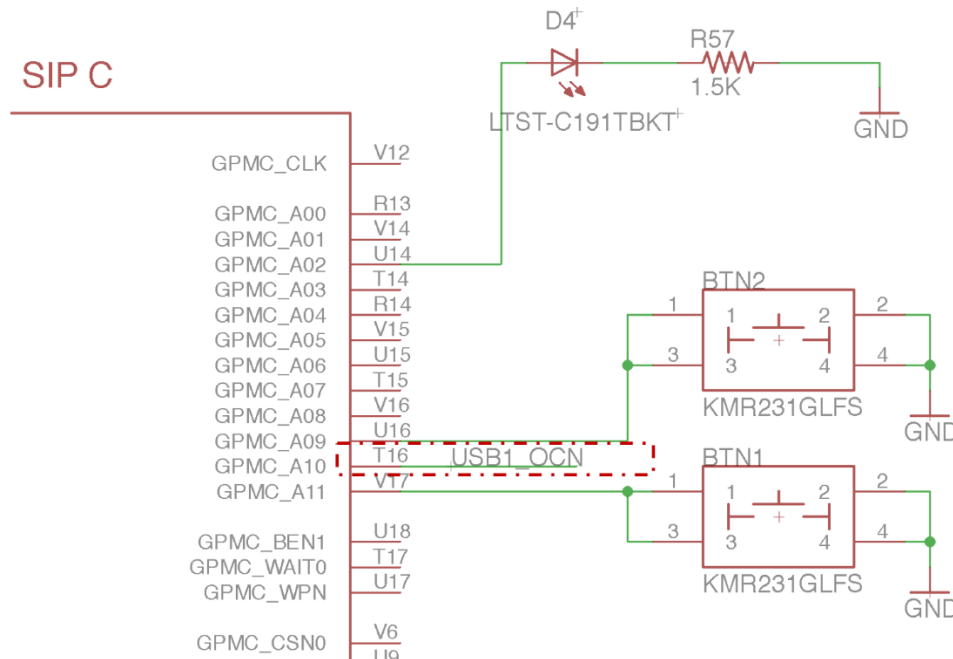
Figure 88 USB1_OCN connection
