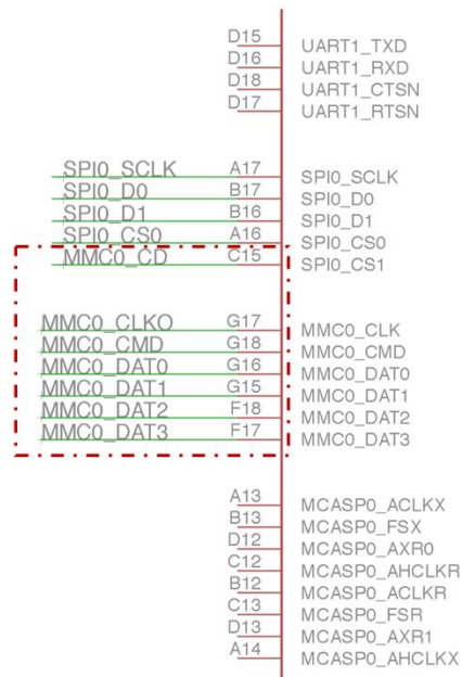
Figure 96 OSD335x SD Card connections
