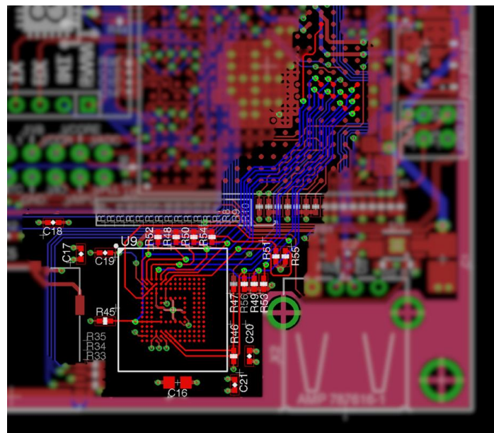
Figure 100 eMMC Layout
