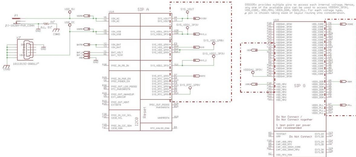
Figure 11 OSD335x schematic for test points on internal power rails and power output pins
