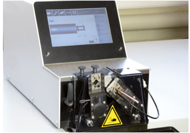
Automatic stripping
