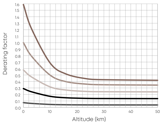
Derating factor
