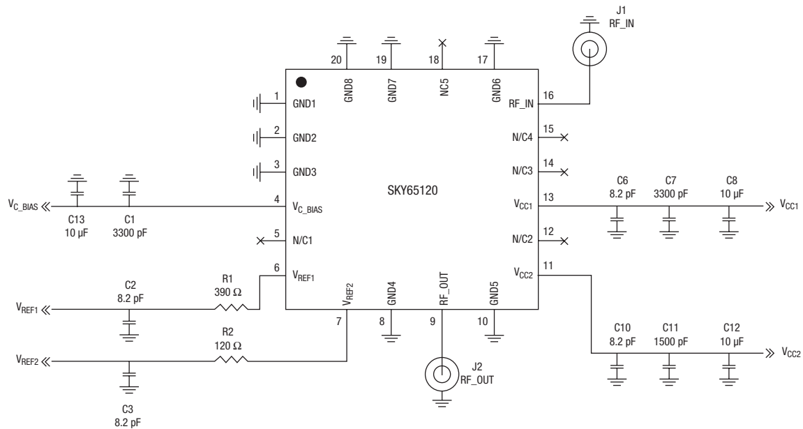
Figure 3. SKY65120 Evaluation Board Schematic
